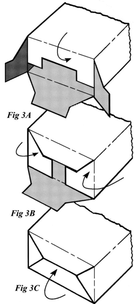
Figure 3—Closing Sequence
